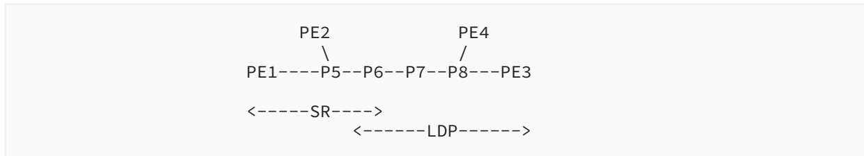
Figure 2: SR and LDP Interworking
